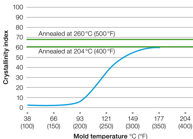
Figure 2: Effect of mold temperature on crystallinity
